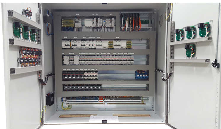
Armoire murale
