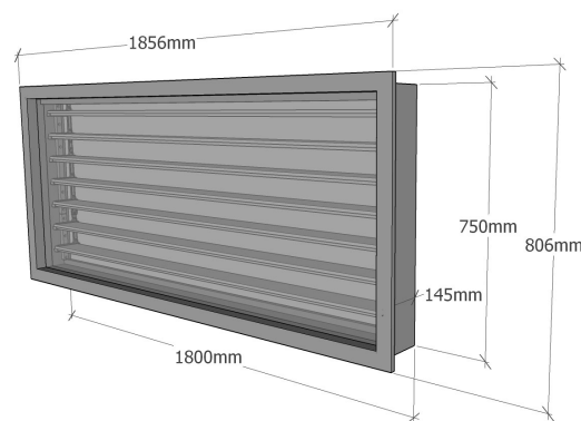
Version L1 (mm)
